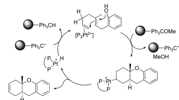
Scheme 1. Proposed catalytic cycle for [Pt 2+ ]-catalyzed polycyclization.
